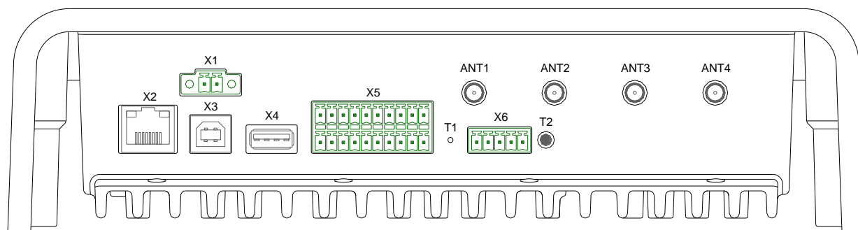
Fig. 2: Connection Overview
