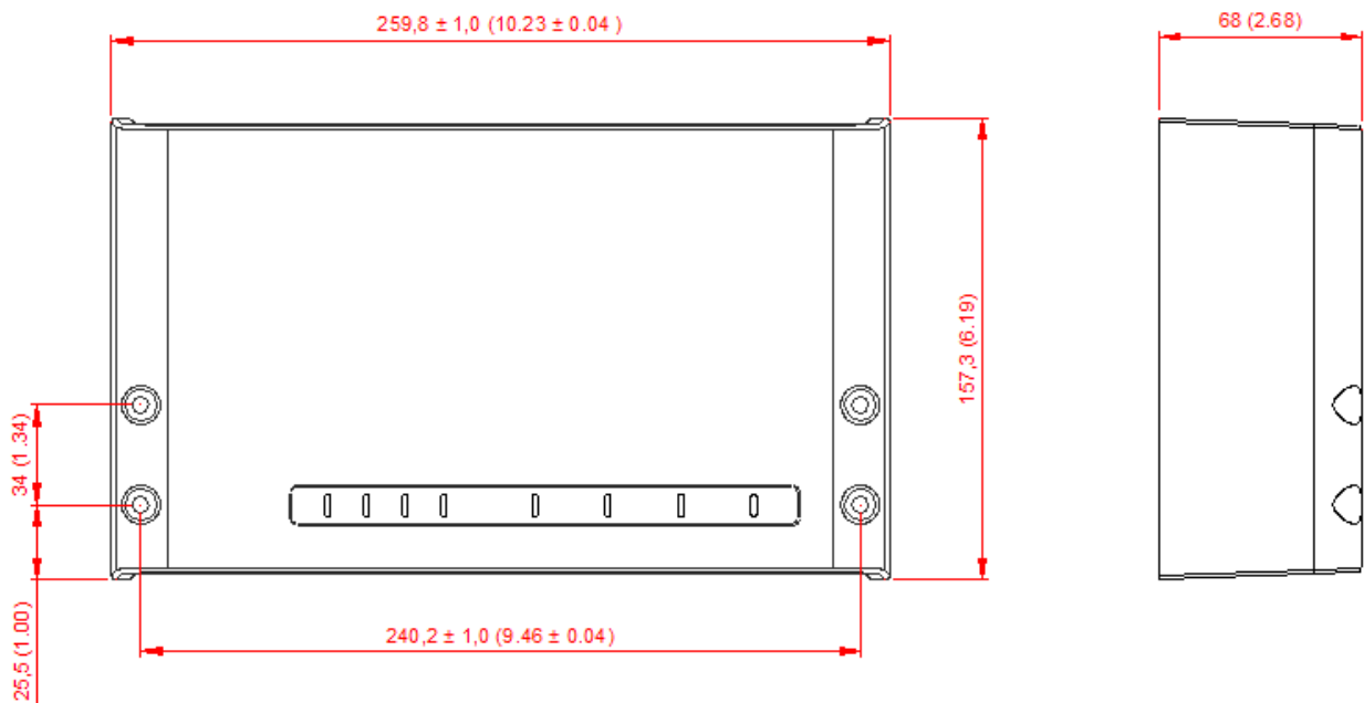
Fig. 1: Installation Drawing
