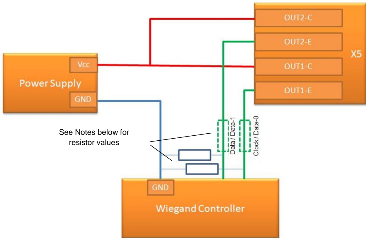
Fig. 12: Wiring Example
